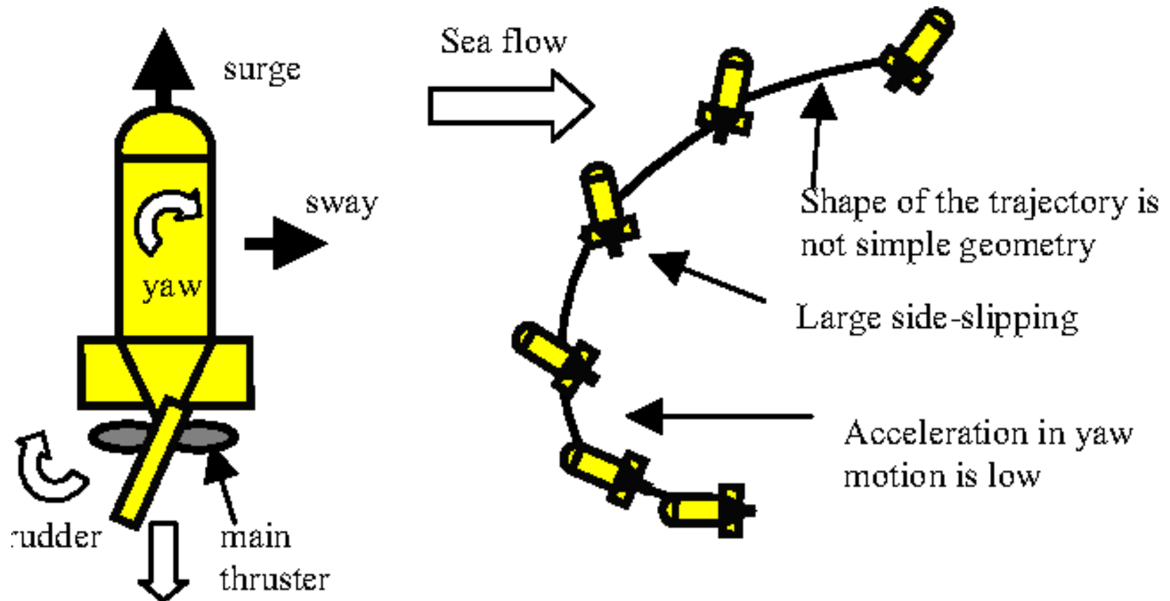
Fig. 1. Configuration of a typical under-actuated underwater vehicle and its motion in strong sea flow.
