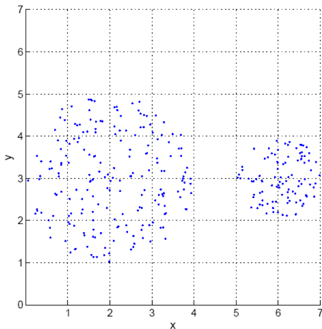
Figure 7.13. Cell-based density.
