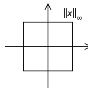
Unit circles
