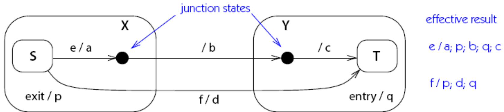
Figure 14-170. Junction pseudostates with multiple actions
