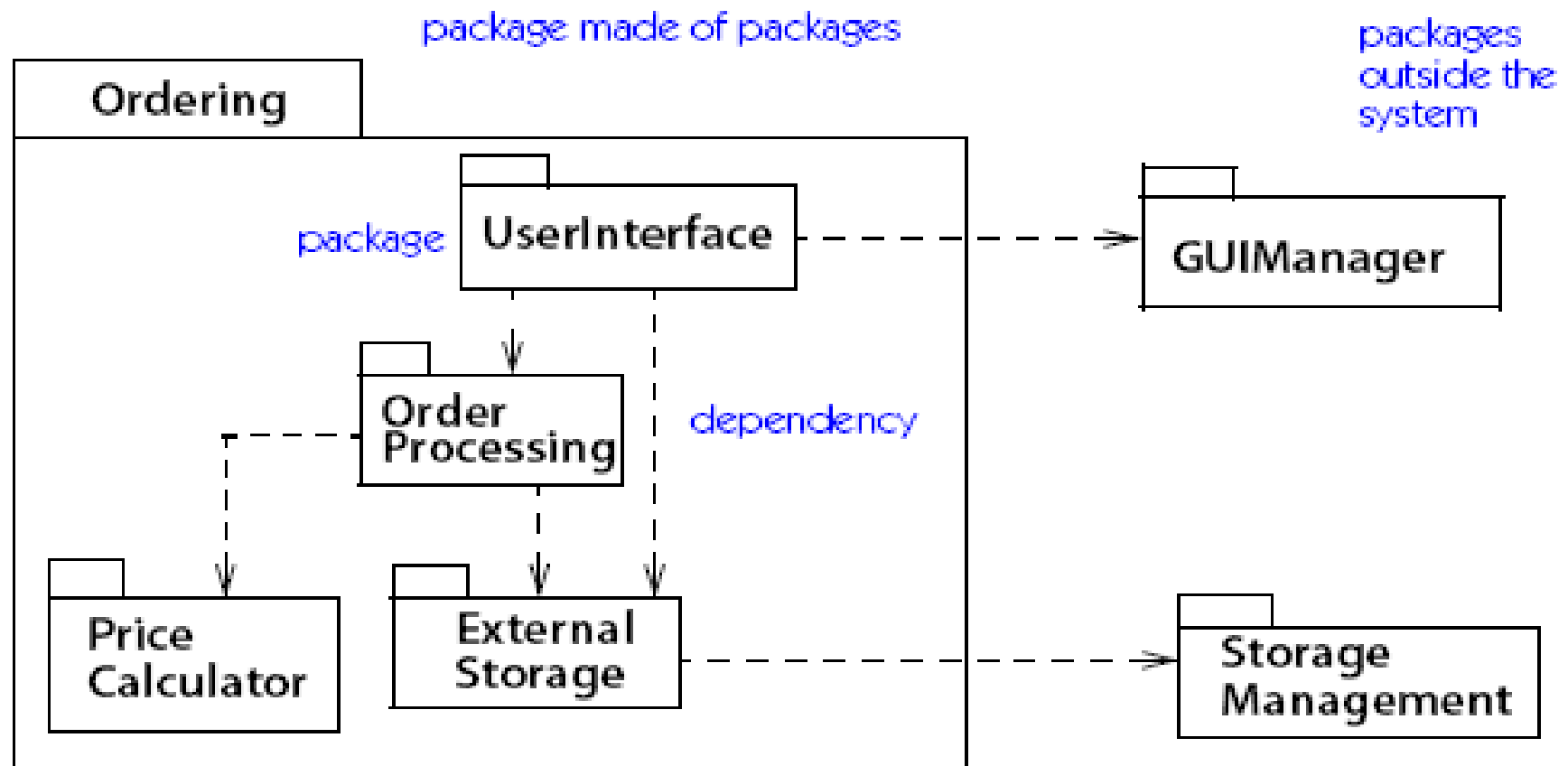
Figure 14-203. Packages and their relationships
