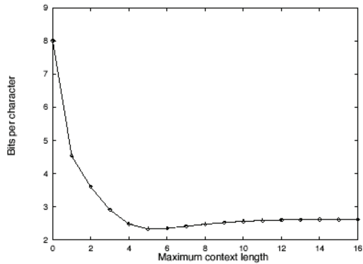
FIGURE 10.12: PPM compression ratio on increasing context length. Computed on Thomas Hardy's text Far from the Madding Crowd .
