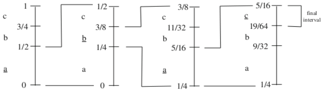
FIGURE 10.11: The algorithmic idea behind Arithmetic coding.
