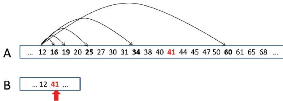
FIGURE 9.4: An example of the Doubling Search paradigm: the two sequences A and B are assumed to have been intersected up to the element 12. The next element in B , i.e. 41, is taken to be exponentially searched in the suffix of A following 12. This search checks A 's elements at distances which are a power of two—namely 1, 2, 4, 8, 16—until it finds the element 60 which is larger than 41 and thus delimits the portion of A within which the binary search for 41 can be confined. We notice that the searched sub-array has size 16, whereas the distance of 41 from 12 in A is 11 thus showing, on this example, that the binary search is executed on a sub-array whose size is smaller than twice the real distance of the searched element.
