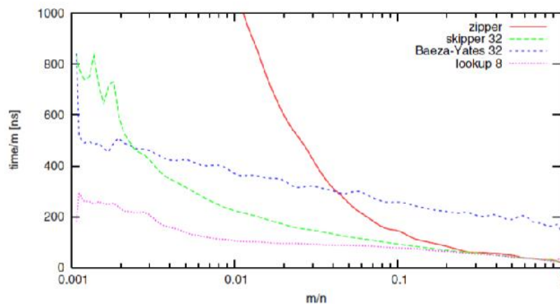
FIGURE 9.6: An experimental comparison among four sorted-set intersection algorithms.
