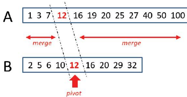
FIGURE 9.3: An example of the Intersection paradigm based on Mutual Partitioning: the pivot is 12, the median element of B .
