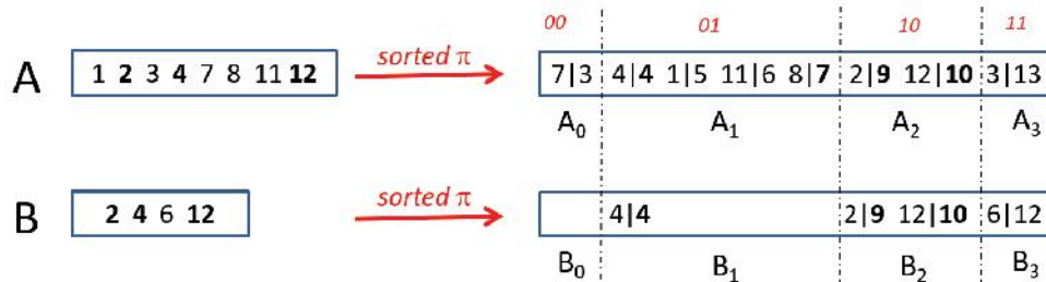
FIGURE 9.5: An example of the Random Permuting and Splitting paradigm. We assume universe U = \{1, \dots, 13\} , set L = 2 and M = 8 , and consider the permutation \pi(x) = 1 + (4x \bmod 13) . So U is partitioned in M/L = 4 buckets identified by the MSB \ell = \lceil \log_2 UL/M \rceil = \lceil \log_2 13 * 2/8 \rceil = 2 bits of the \pi -image of each element. Recall that every \pi -image is represented in \log_2 u = 4 bits, so that \pi(1) = 5 = (0101)_2 and its 2 MSB are 01. The figure shows in bold the elements of A \cap B , moreover it depicts for the sake of exposition each docID as the pair x|\pi(x) and, on top of every sublist, shows the 2 MSBs. In the example only three buckets of B are unempty, so we intersect only them with the corresponding ones of A , so that we drop the sublist A_1 without scanning it. The result is \{4|4, 2|9, 12|10\} , that gives A \cap B by dropping the second \pi -component: namely, \{2, 4, 12\} .
