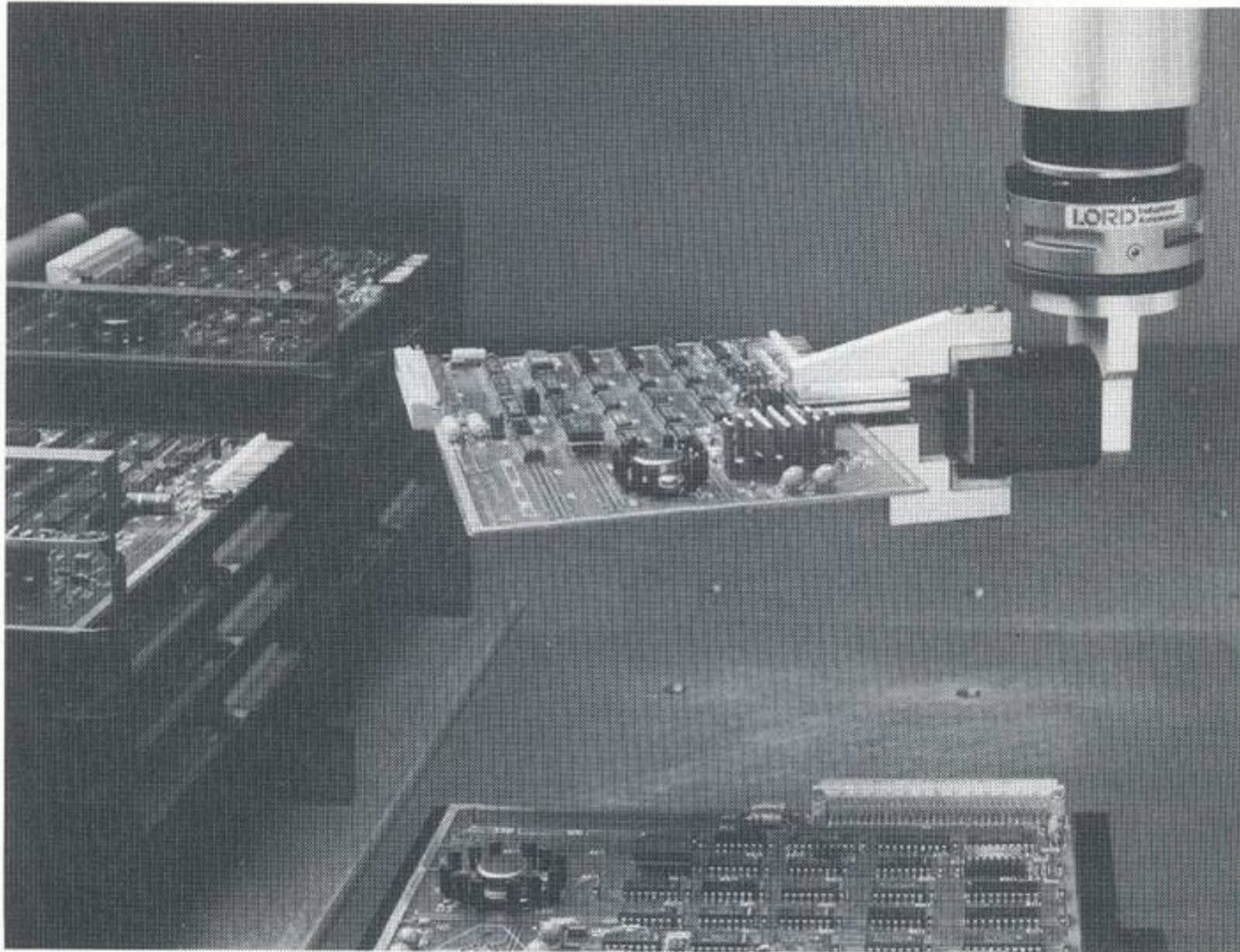
Figure 4.22 A force sensor is used to measure the force exerted by the robotic arm on the PCB.
